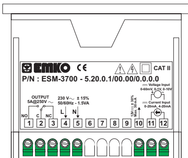
Device Label for Universal Process Input, 230V ~ Supply Voltage Input and Alarm Relay Output
