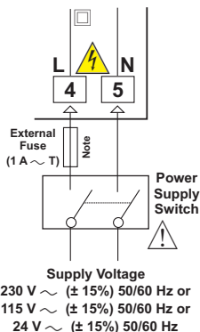
Connection of Supply Voltage Input
