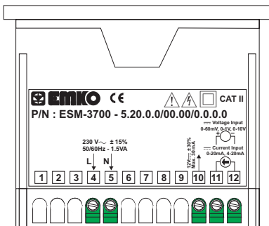
Device Label for Universal Process Input, 230V ~ Supply Voltage Input and Without Alarm Output
