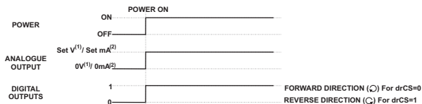
Figure-4.3 Power On Behaviour (Strt=2)
