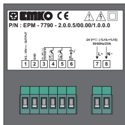
Device Label for (0/2...10V \sim ) Output and 24V \sim Supply Voltage Input
