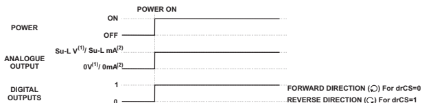
Figure-4.2 Power On Behaviour (Strt=1)
