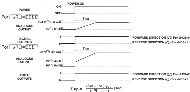
Figure-4.4 Power On Behaviour (Strt=3)
