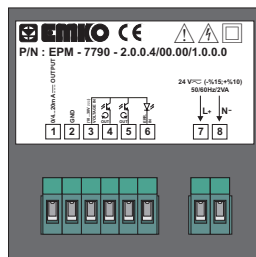
Device Label for (0/4...20mA \sim ) Output and 24V \sim Supply Voltage Input
