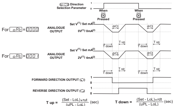
Figure-4.6 Motor Direction Change (lbtn=3)
