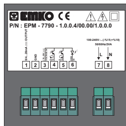
Device Label for (0/4...20mA \sim ) Output and 100-240V \sim Supply Voltage Input
