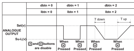
Figure-4.5 Increment and Decrement Button Functional Usage
