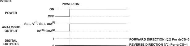
Figure-4.1 Power On Behaviour (Strt=0)
