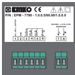
Device Label for (0/2...10V \sim ) Output and 100-240V \sim Supply Voltage Input
